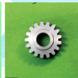
Leno Pinion Gear 17 Teeth Steel Item Code GE 04 613
