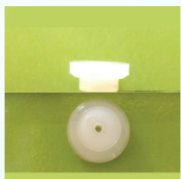
Poppet valve Plunger top Sulzer L5500 Item Code GE 05 517
